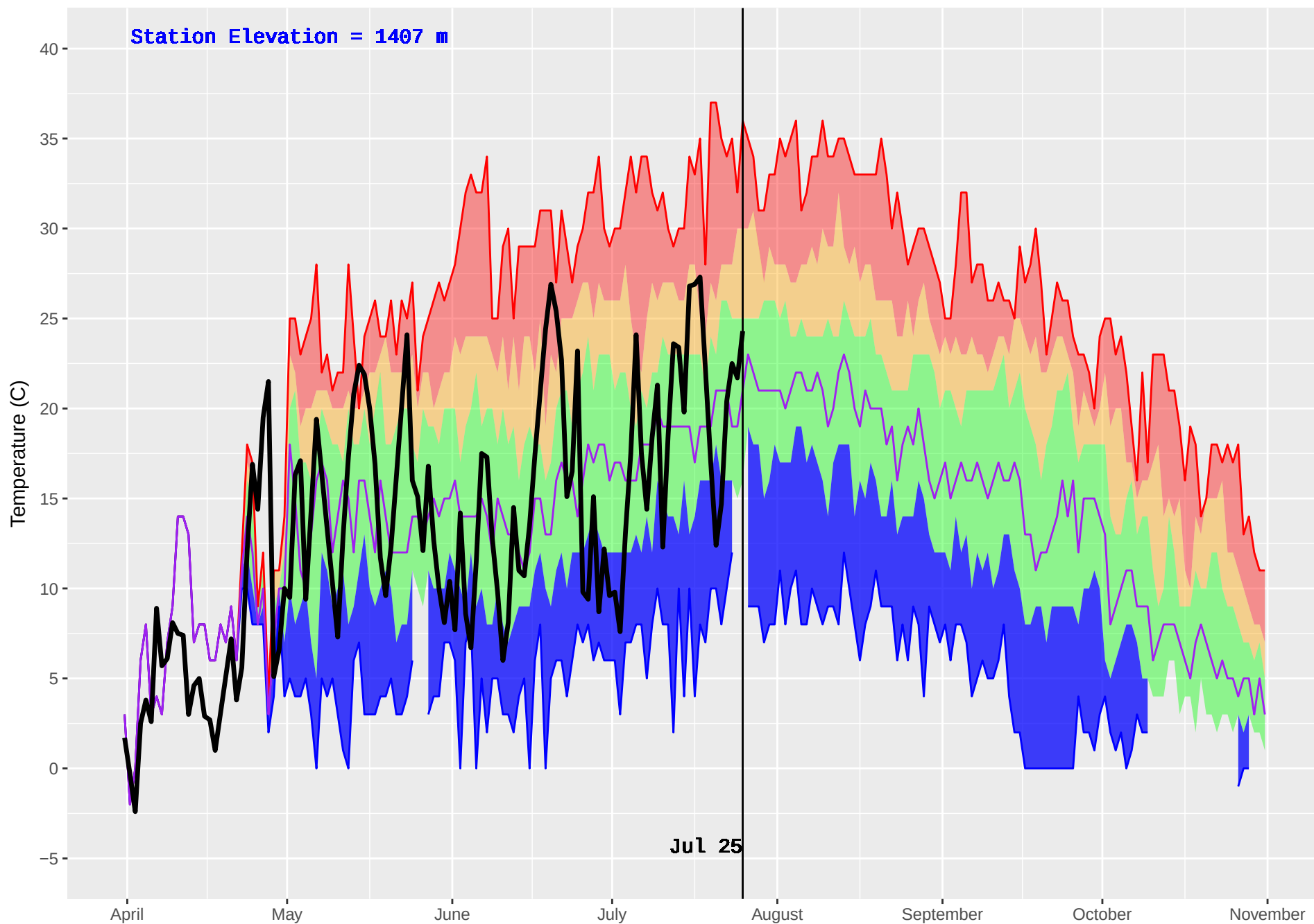
THYNNNE (279) : Historical (1977–2016) and Current (2018) Noon Temperature
