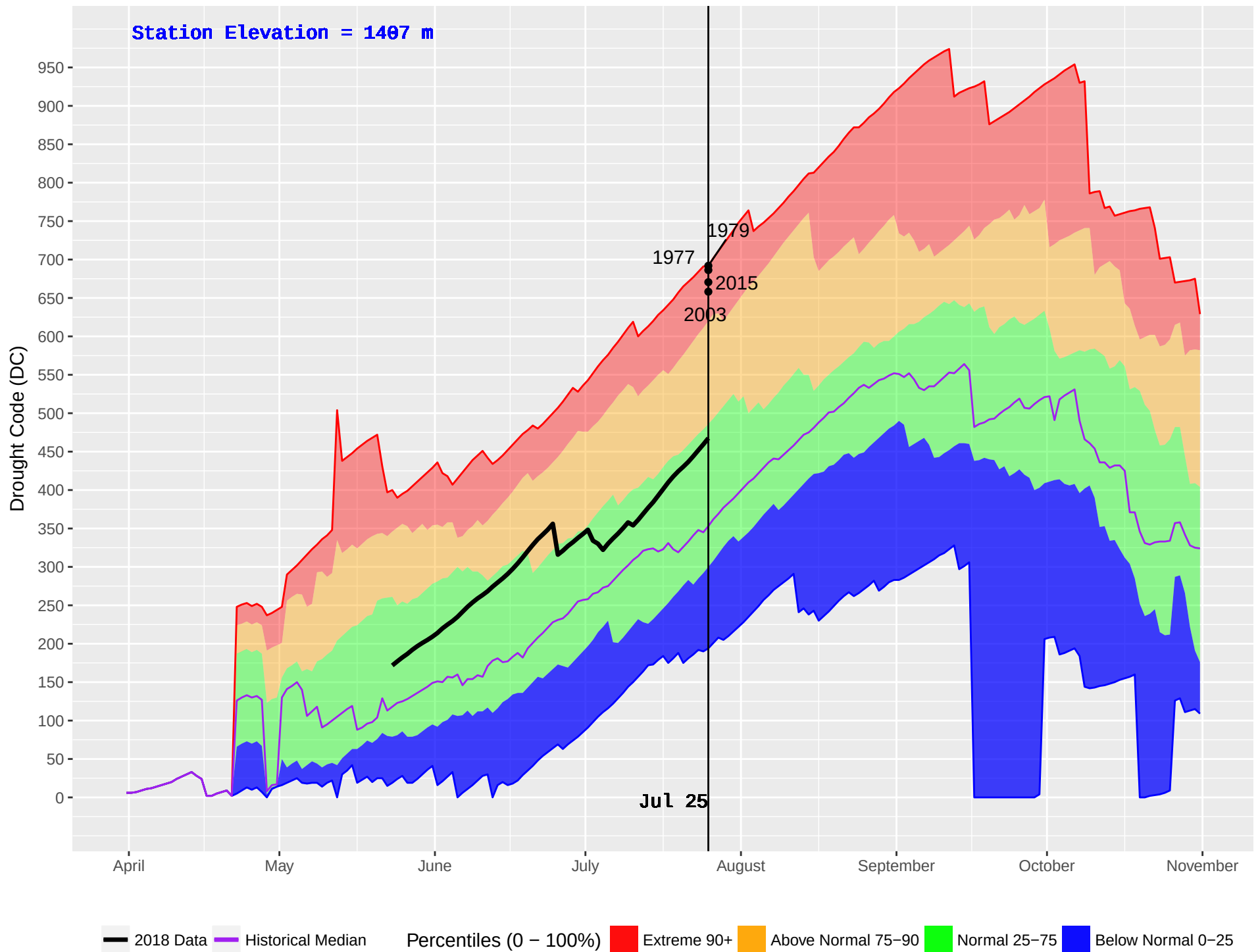
THYNNE (279) : Historical (1977–2016) and Current (2018) Noon Drought Code (DC)
