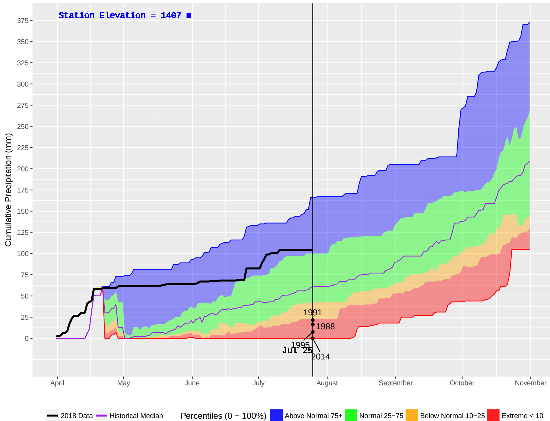
THYNNE (279) : Historical (1977–2016) and Current (2018) Noon Cumulative Precipitation
