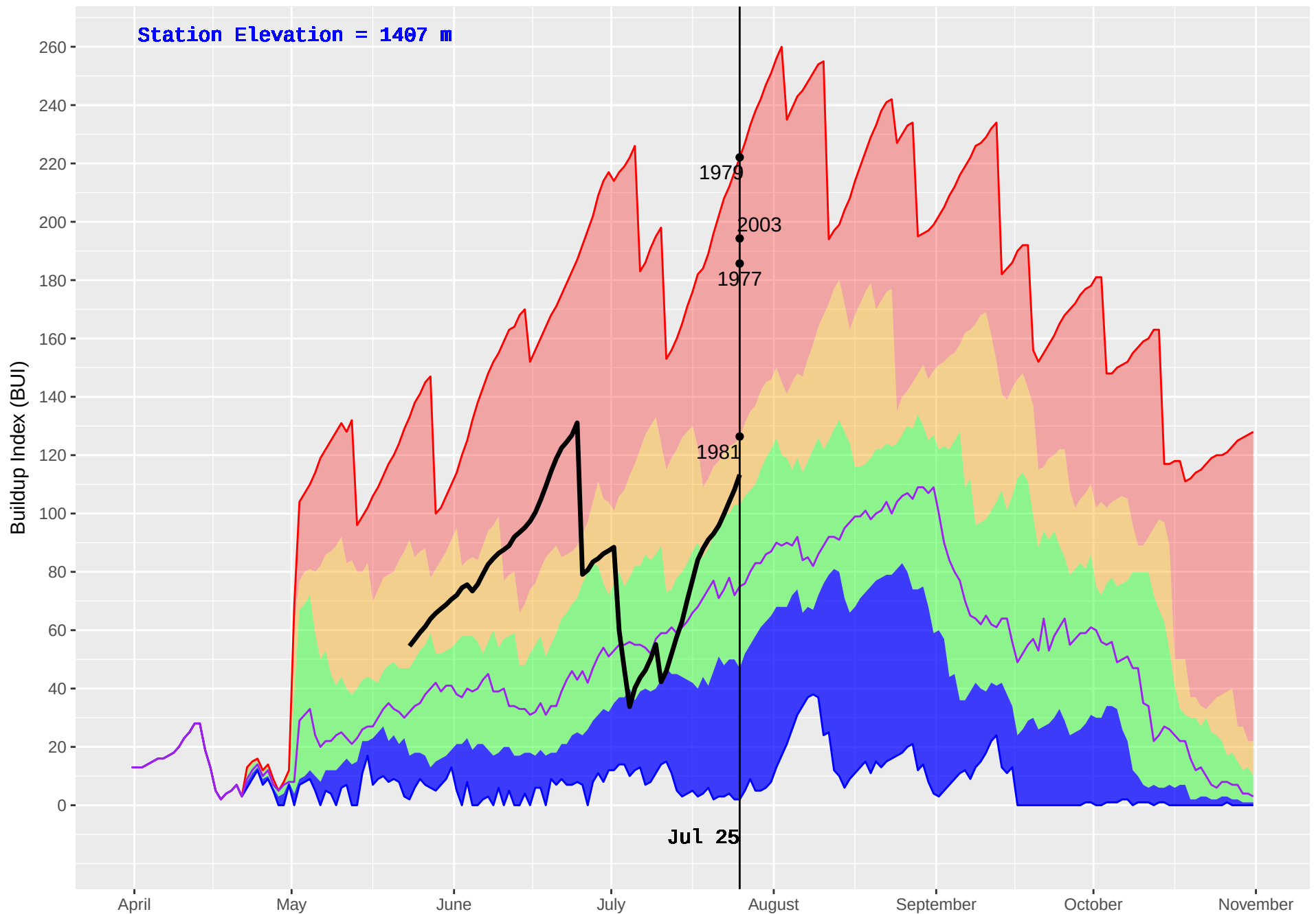
THYNNE (279) : Historical (1977–2016) and Current (2018) Noon Buildup Index (BUI)
