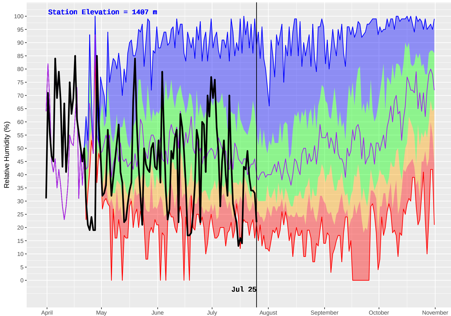
THYNNE (279) : Historical (1977–2016) and Current (2018) Noon Relative Humidity
