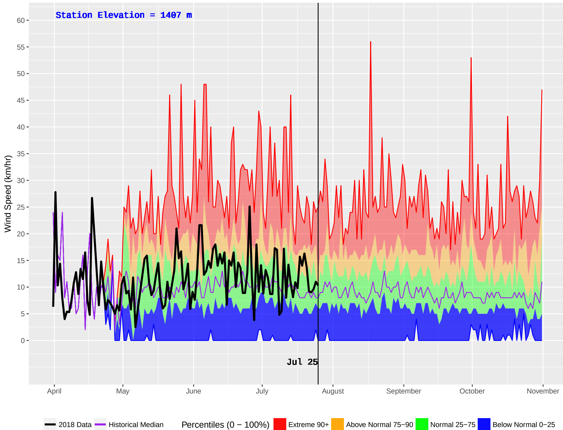
THYNNNE (279) : Historical (1977–2016) and Current (2018) Noon Wind Speed
